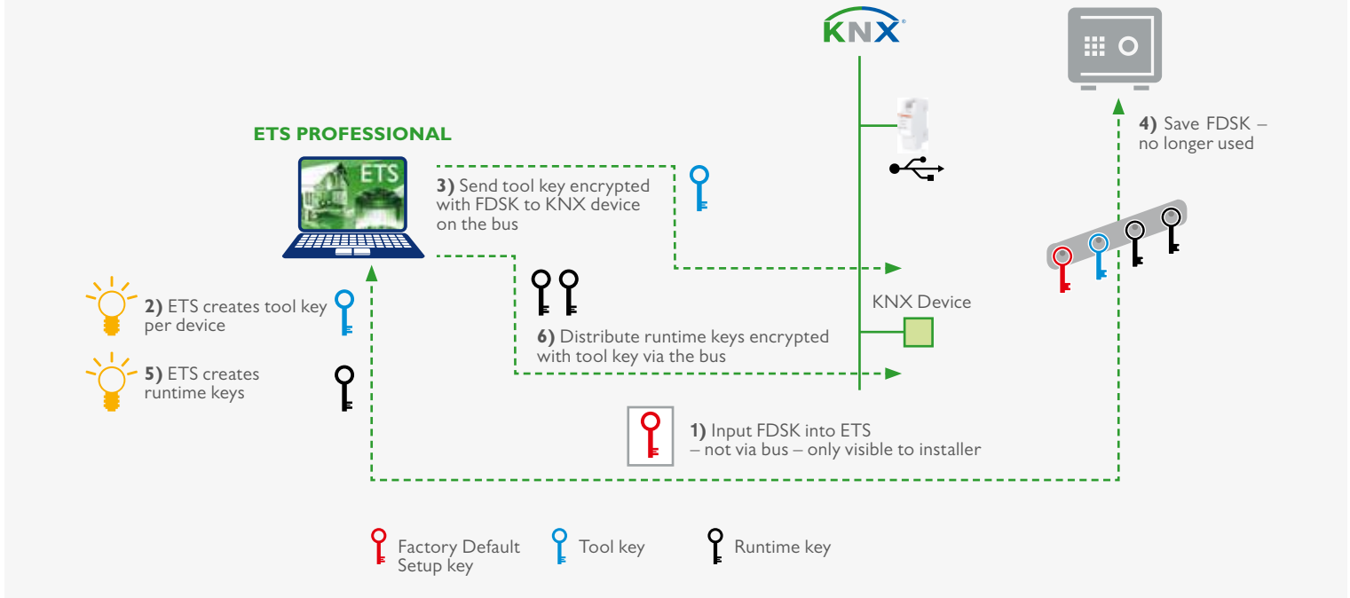
Procedure for securing KNX devices
