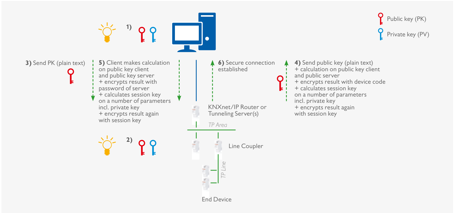
Setting up a KNX IP Secure Connection
